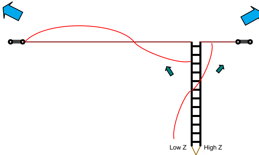
Energy easily coupled at 18 MHz to the 3.7 MHz element
