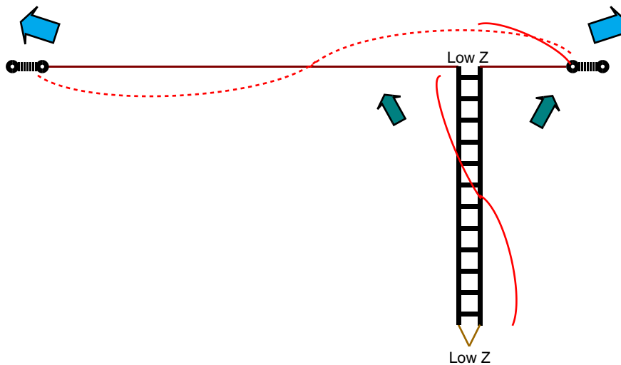
Energy easily coupled at 21 MHz
